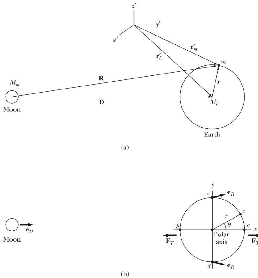
Figure 5.6: Geometry used to determine the forces on a volume of water of mass m , located on the surface of the Earth.
