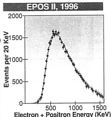
A signal fades. The original EPOS experiment revealed a peak in the energy of electron-positron pairs generated by collisions of uranium and thorium ions. In later EPOS measurements, a peak reappeared but at varying energies. The most recent studies, from EPOS II and APEX, show no sign of a peak. The upper APEX spectrum reproduces the original EPOS analysis.
