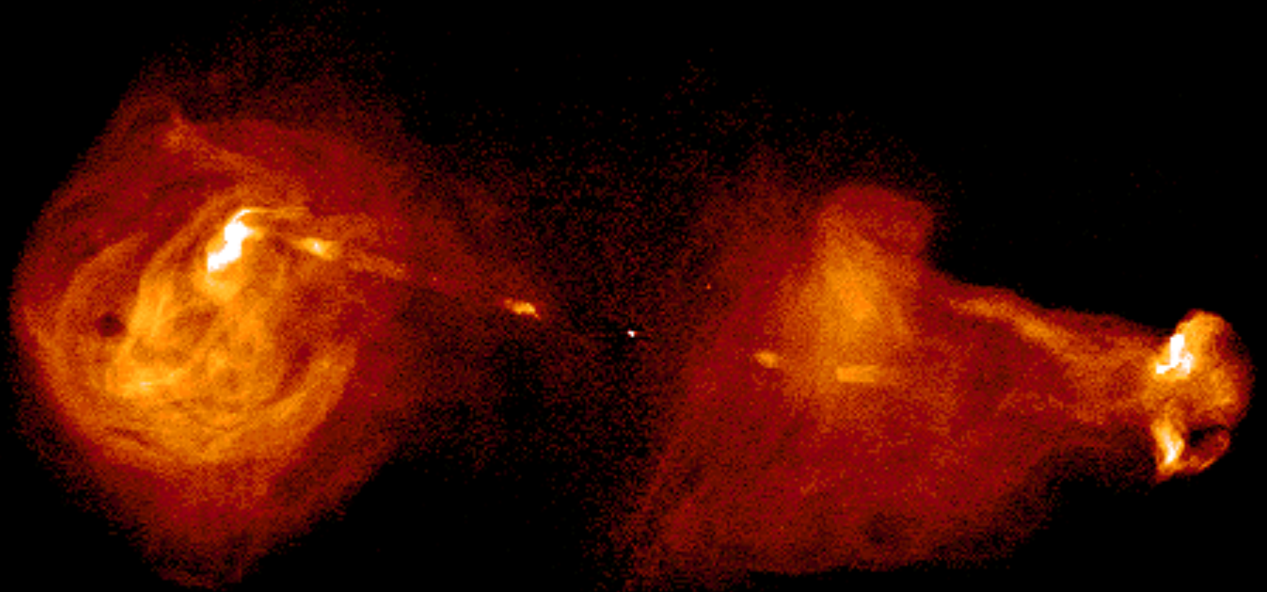
Radio Galaxy 3C353 VLA 3.6cm image (c) NRAO 1996
