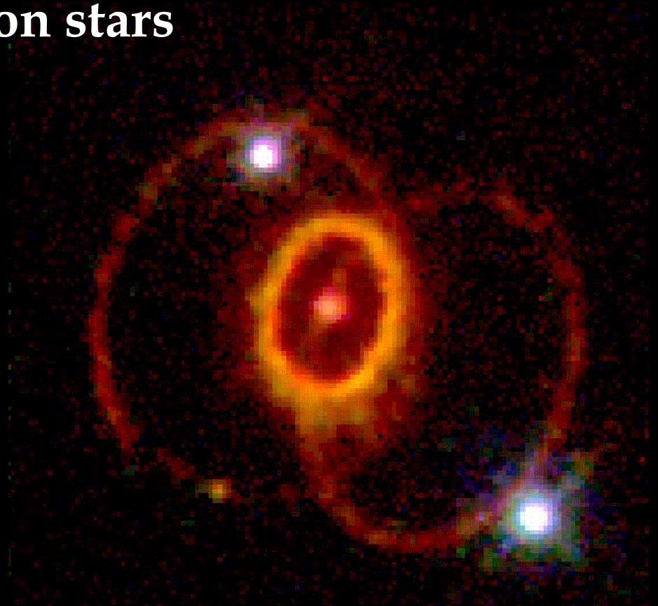
The remnant of supernova 1987A in the Large Magellanic Cloud, seen by the Hubble Space Telescope in 1995 ( NASA/STScI ).
