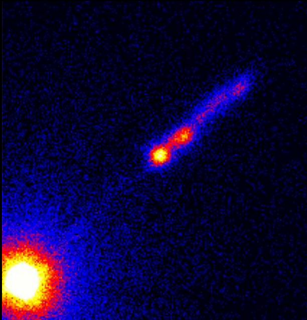
X ray image, by the NASA Chandra X-ray observatory (CXO).
