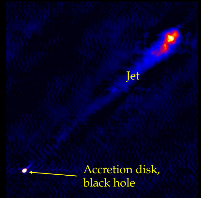
Radio image, by the Multi-Element Radio Linked INterferometer (MERLIN).
