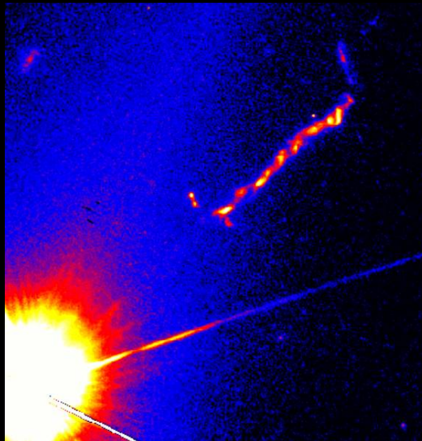
Visible-light image, by the NASA Hubble Space Telescope (HST).
